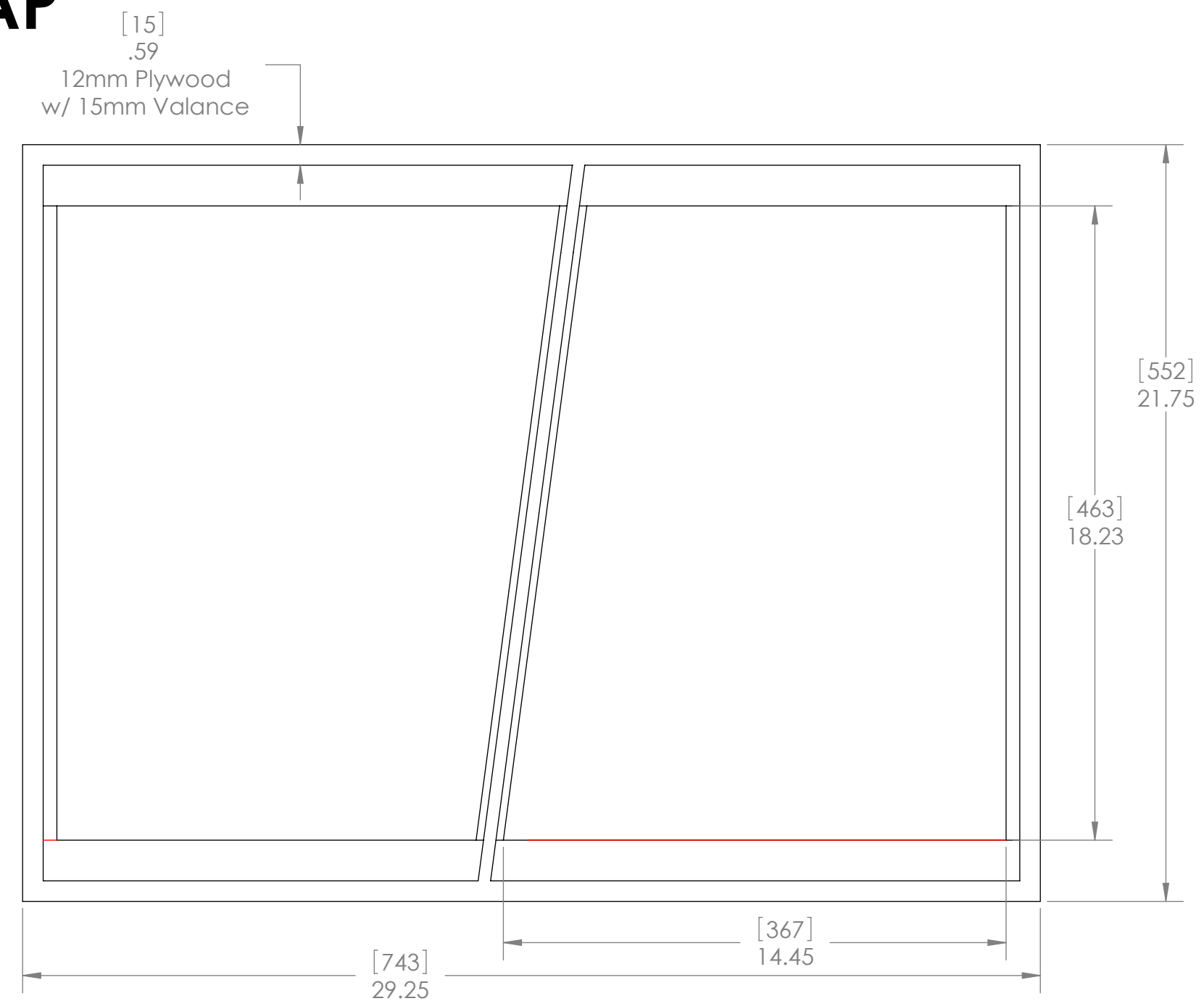
Top View
